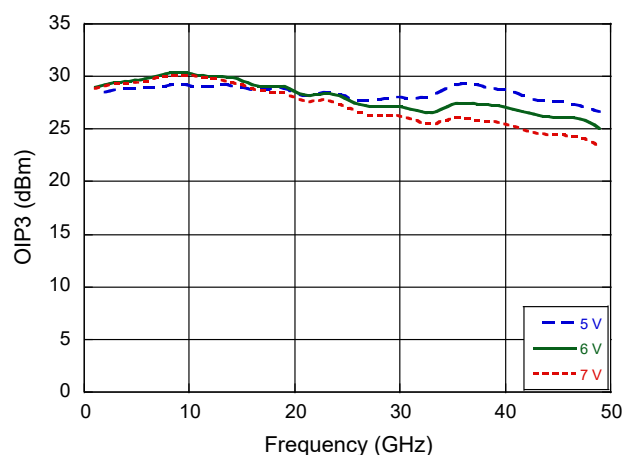
OIP3 at T_A = 25^\circ\text{C}
